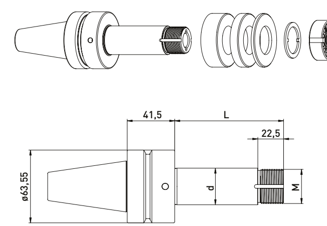
类似 SK40 with flat contact face
