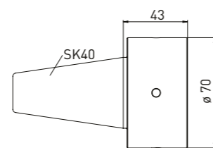
Order No. Name 350130039 Adapter SK40 on Rollomatic ø25
