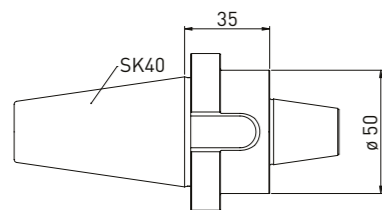
Order No. Name 350130035 Adapter SK40 on ANCA taper ø30
