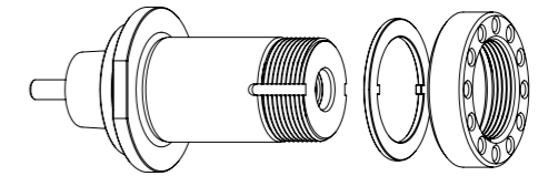
GWA manual HSK-F40 // \varnothing 31,75 mm // without RS
