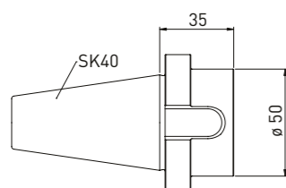
Order No. Name 350130042 Adapter SK40 on Strausak Promat
