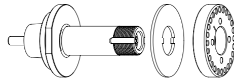
GWA manual HSK-F40 // \varnothing 20 mm // without RS
